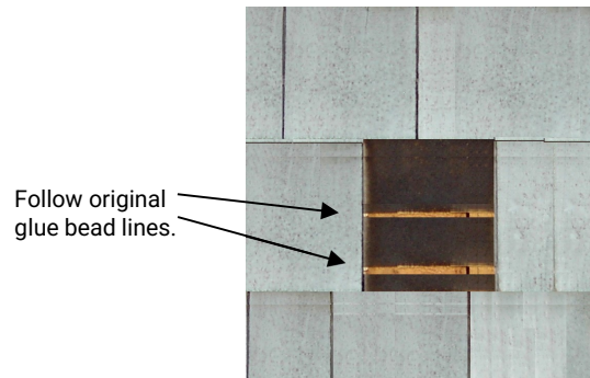
(Remove shingle)
